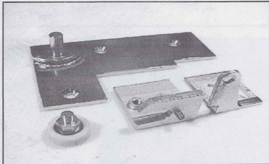
12-15-104 Pivot & Guide, A/L LH 12-15-105 Pivot & Guide, A/L RH (Shown)
